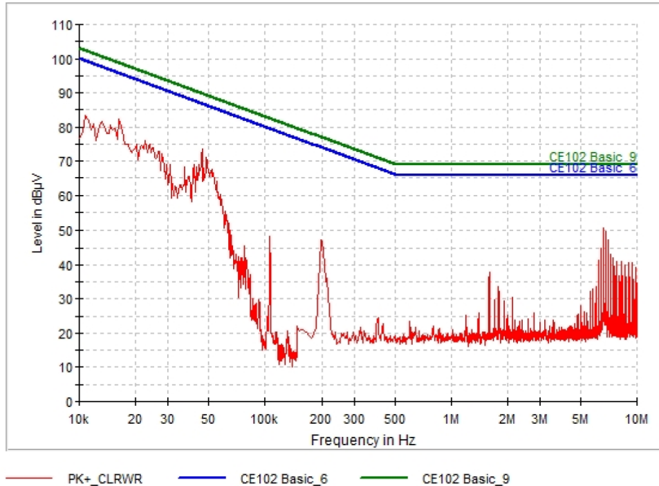
Fig. 16.1 MIL-STD-461F CE102 Result OFD1200A28, 115V, N
