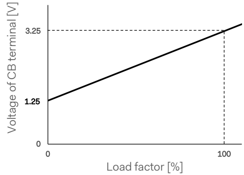
Fig. 5.10 CB terminal voltage vs output current
