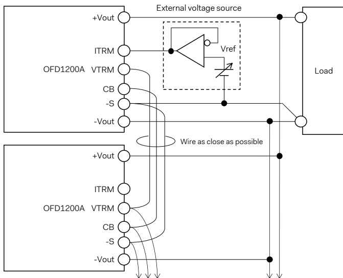
Fig. 5.9 Example of connecting constant current circuit with an external voltage
