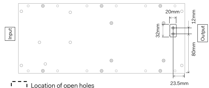
Fig. 1.2 The Location of open hole on aluminium baseplate (Bottom view)
