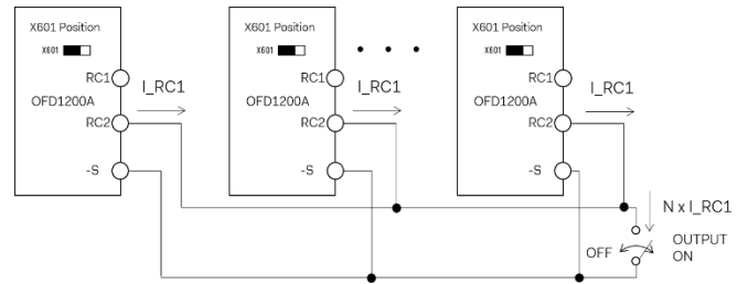
Fig. 5.6 Example of connecting remote ON/OFF circuit
