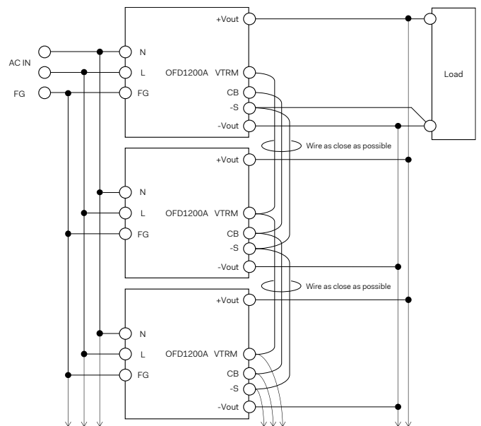
Fig. 5.3 Example of wiring for parallel operation
