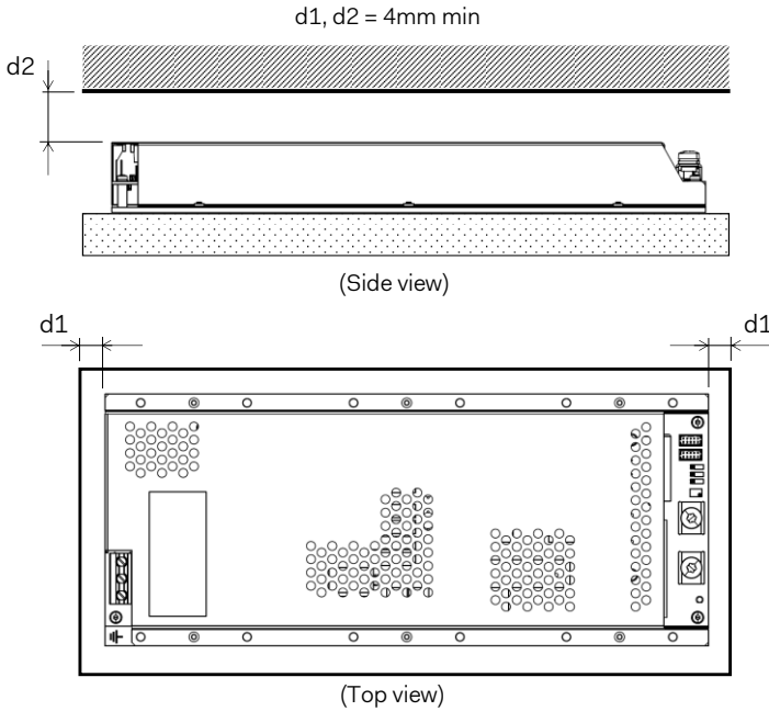
Fig. 1.3 Isolation distance
