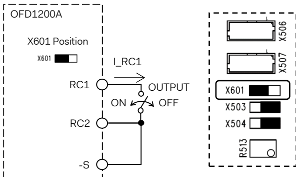
(c) Change position of X601 (Negative logic)
