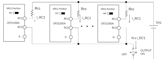
Fig. 5.7 Example of connecting remote ON/OFF circuit
