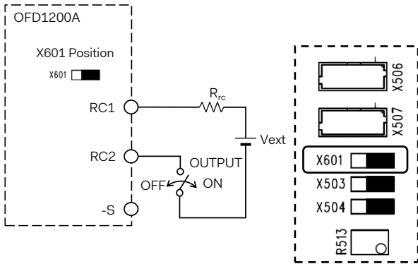
(a) Use external voltage source (Positive logic)
