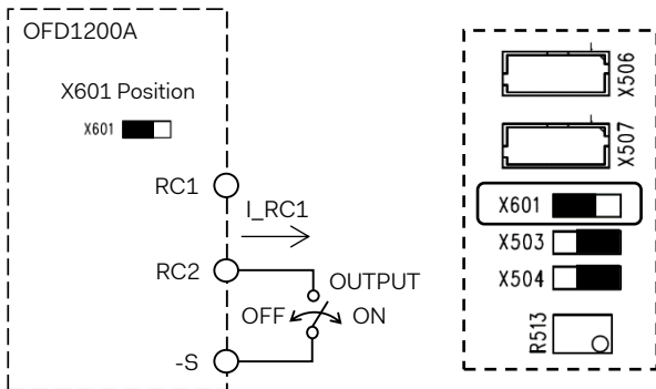
(b) Change position of X601 (Positive logic)
