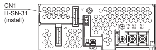
Fig.5.15 Front view of option -W1 (PJMA1000F)
