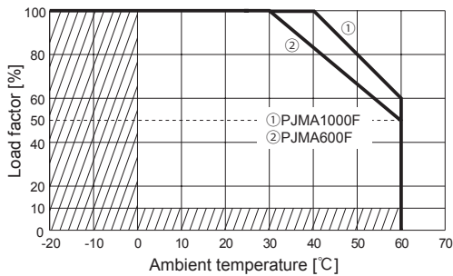
Fig.5.21 Ambient temperature derating curve for PJMA600F and PJMA1000F (Option-F4)
