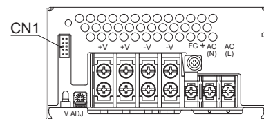
Fig.5.5 Front view of option -R (PJMA600F)
