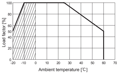
Fig.5.20 Ambient temperature derating curve for PJMA300F (Option-F4)
