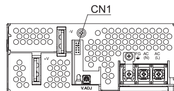
Fig.5.6 Front view of option -R (PJMA1000F)
