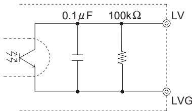
Fig.5.17 LV internal circuit
