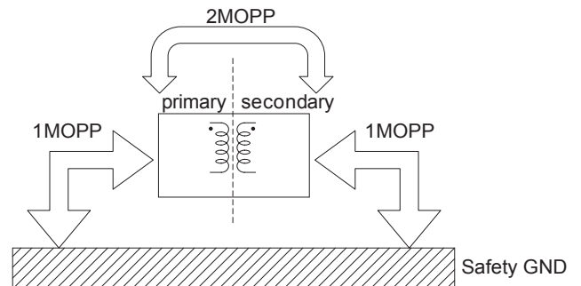
Fig.5.23 Medical Isolation Grade
