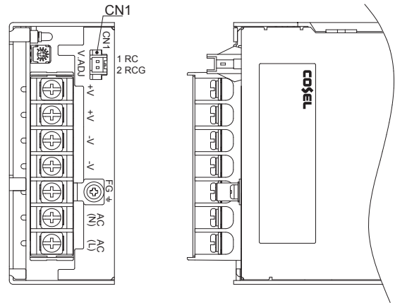
Fig.5.4 Example of option -R (PJMA300F)
