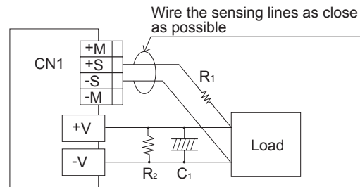
Fig.5.19 When using remote sensing function
