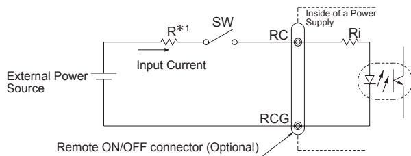
Fig.5.3 Example of using a remote ON/OFF circuit
