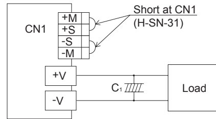
Fig.5.18 When not using remote sensing function
