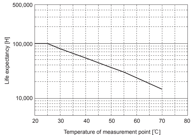
Fig.5.22 Life Expectancy of fan R(t)=90% (-F4)
