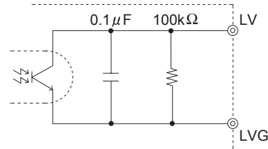
Fig.5.10 LV internal circuit
