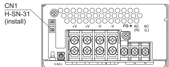
Fig.5.14 Front view of option -W1 (PJMA600F)
