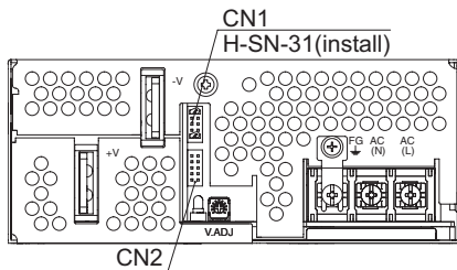
Fig.5.8 Front view of option -W (PJMA1000F)
