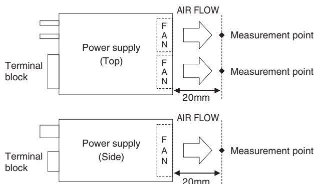
Fig.3.3 Temperature of measurement point for fan lifetime (PJMA1000F)
