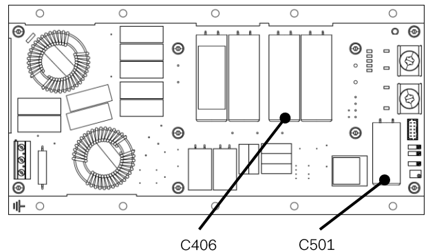
Fig. 6.1 Temperature measuring point for Life expectancy
