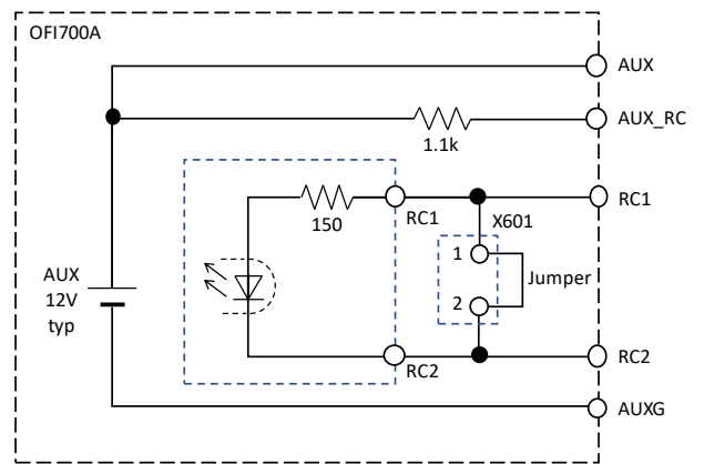
Fig. 4.3 Internal circuit diagram of Remote Control
