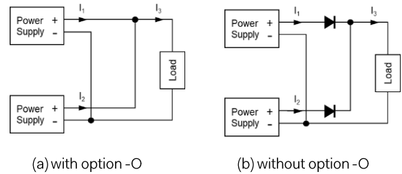
Fig. 5.2 example of 1+1 Redundancy operation
