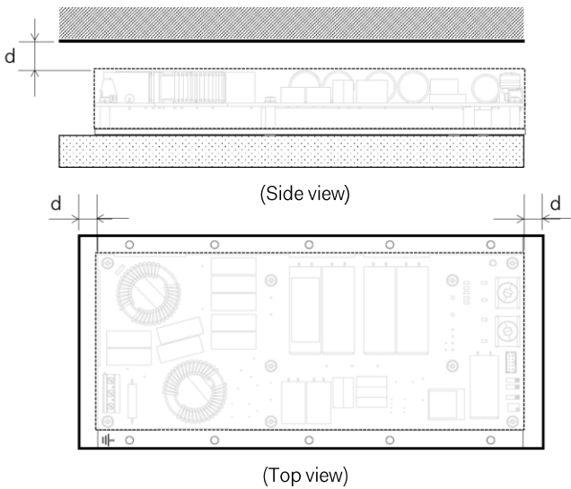
Fig. 1.3 Isolation distance
