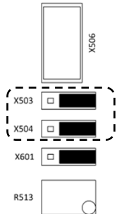
Fig. 4.5 X503 and X504 Jumper position
